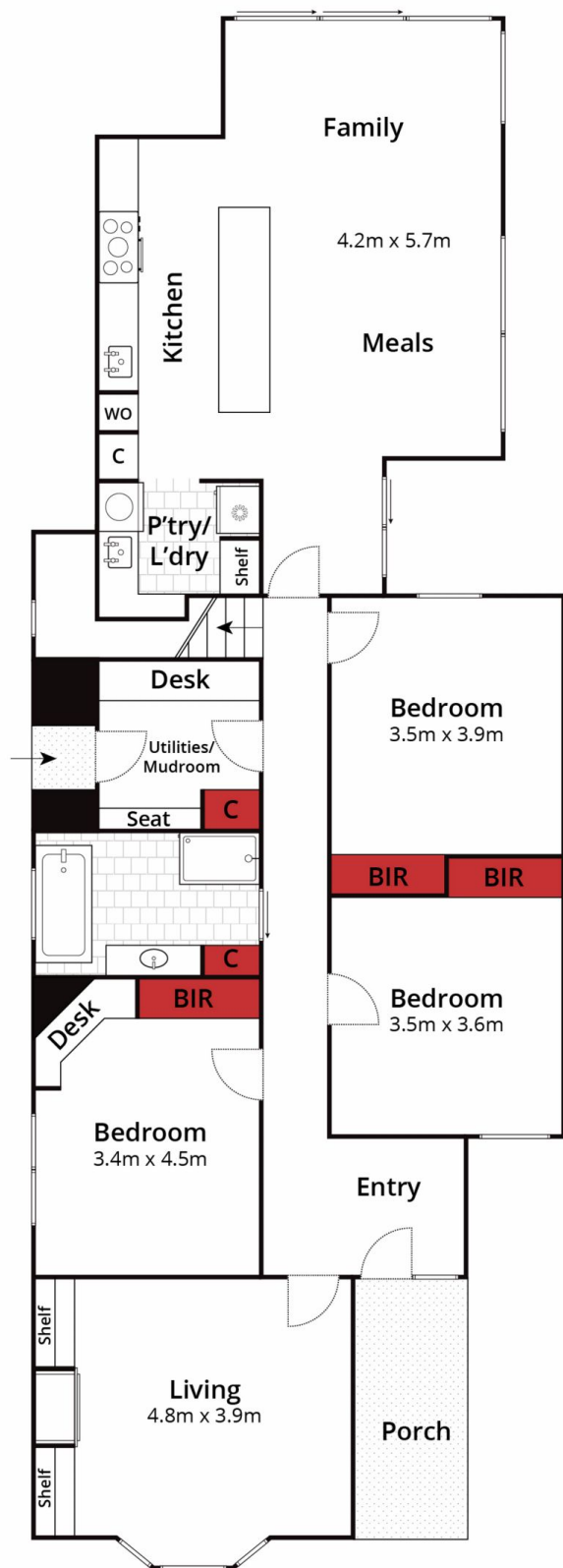
Ground Floor
