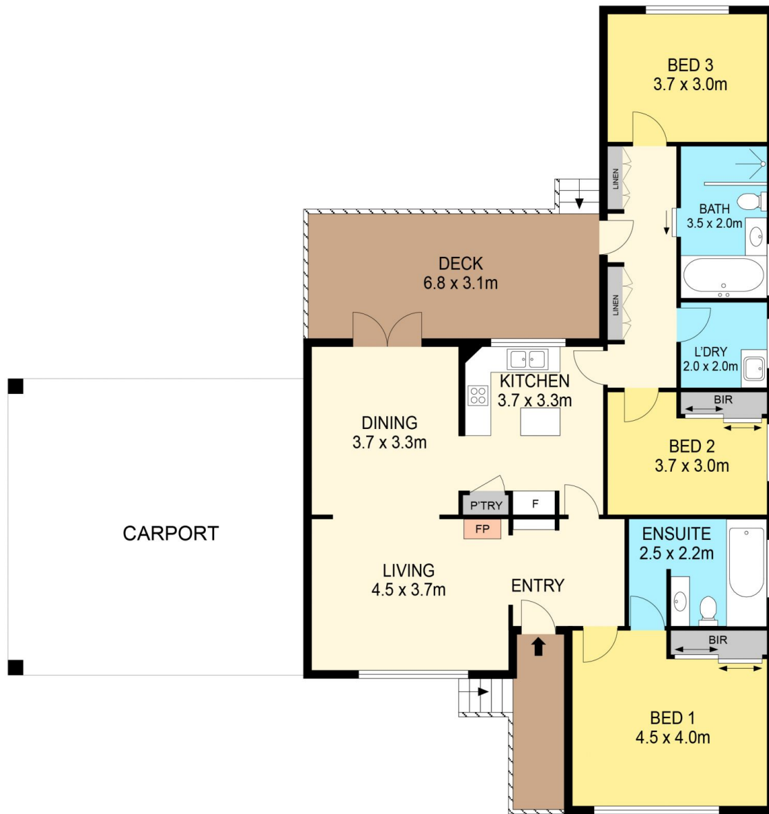
FLOOR PLAN
